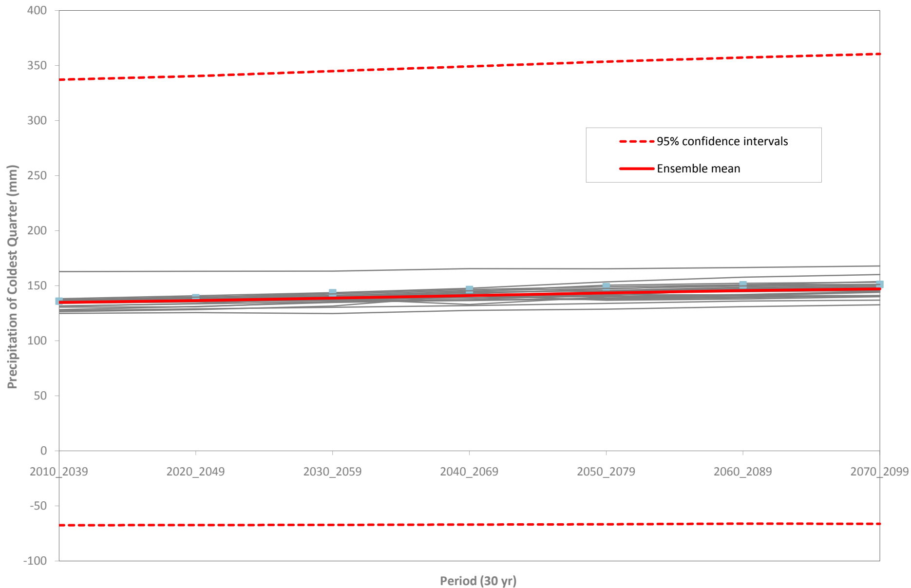
Precipitation of Coldest Quarter (Confidence Intervals)
