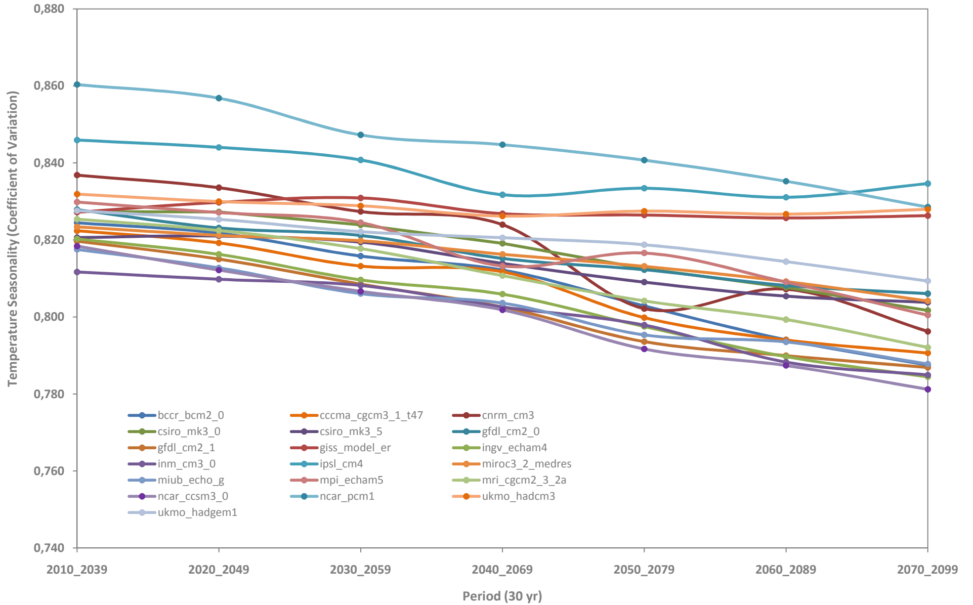
Temperature Seasonality (Coefficient of Variation)
