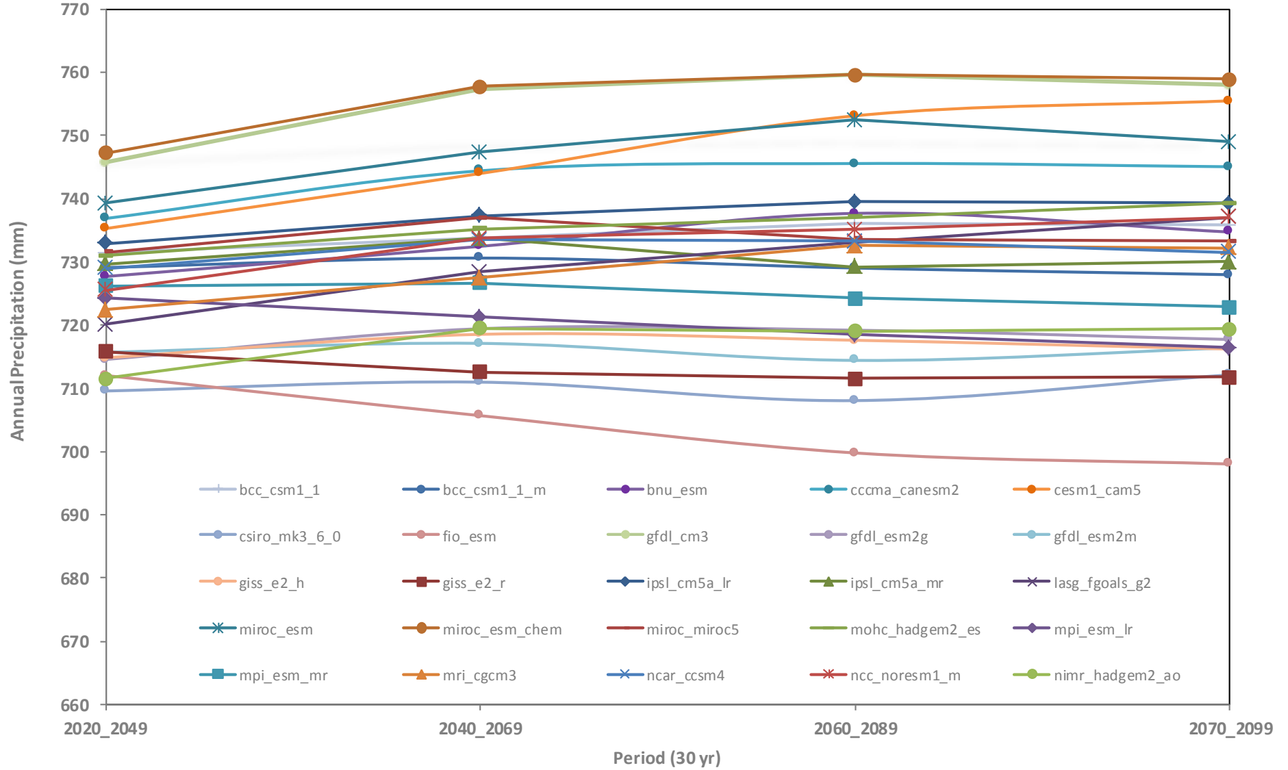
Annual Precipitation
