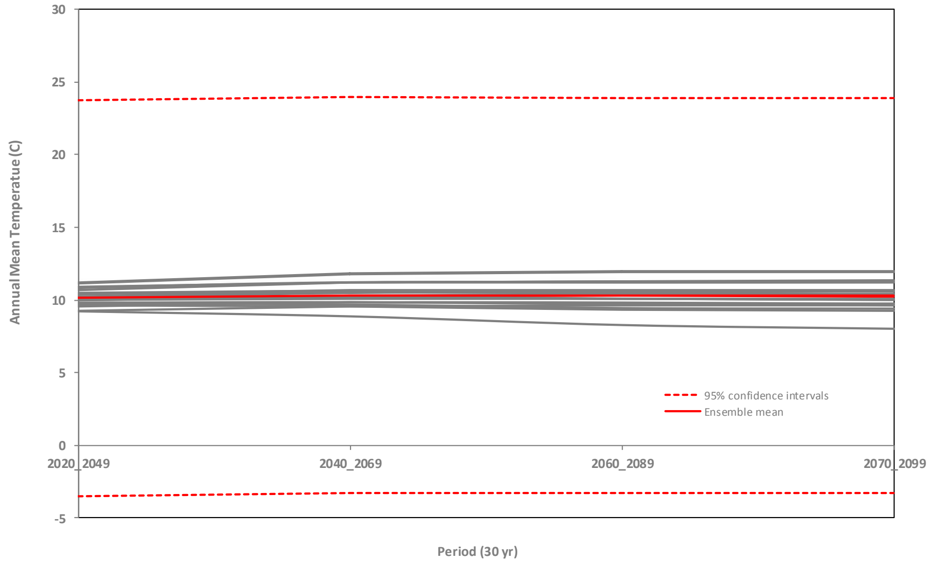
Annual Mean Temperature (Confidence intervals)
