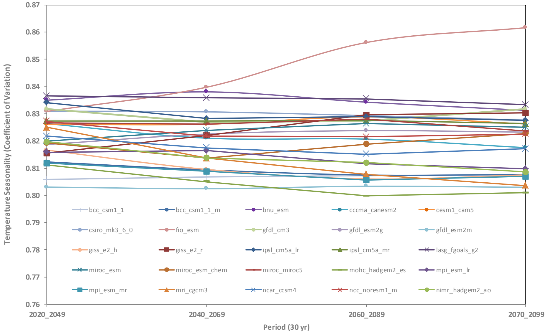
Temperature Seasonality (Coefficient of Variation)
