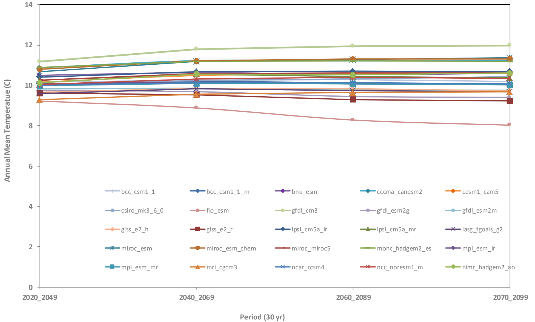
Annual Mean Temperature
