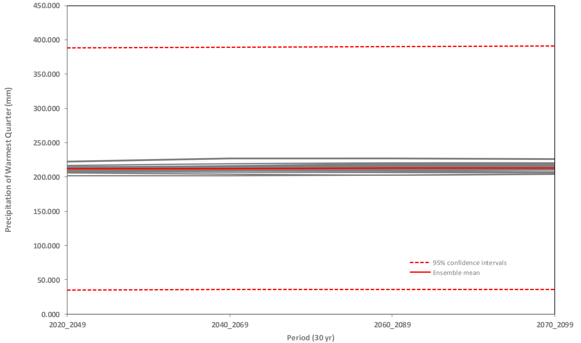
Precipitation of Warmest Quarter (Confidence intervals)
