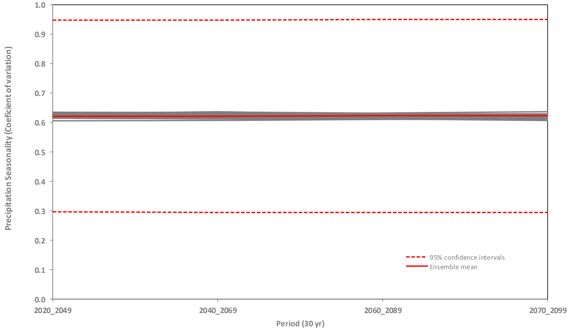
Precipitation Seasonality (Coefficient of variation) Confidence Intervals
