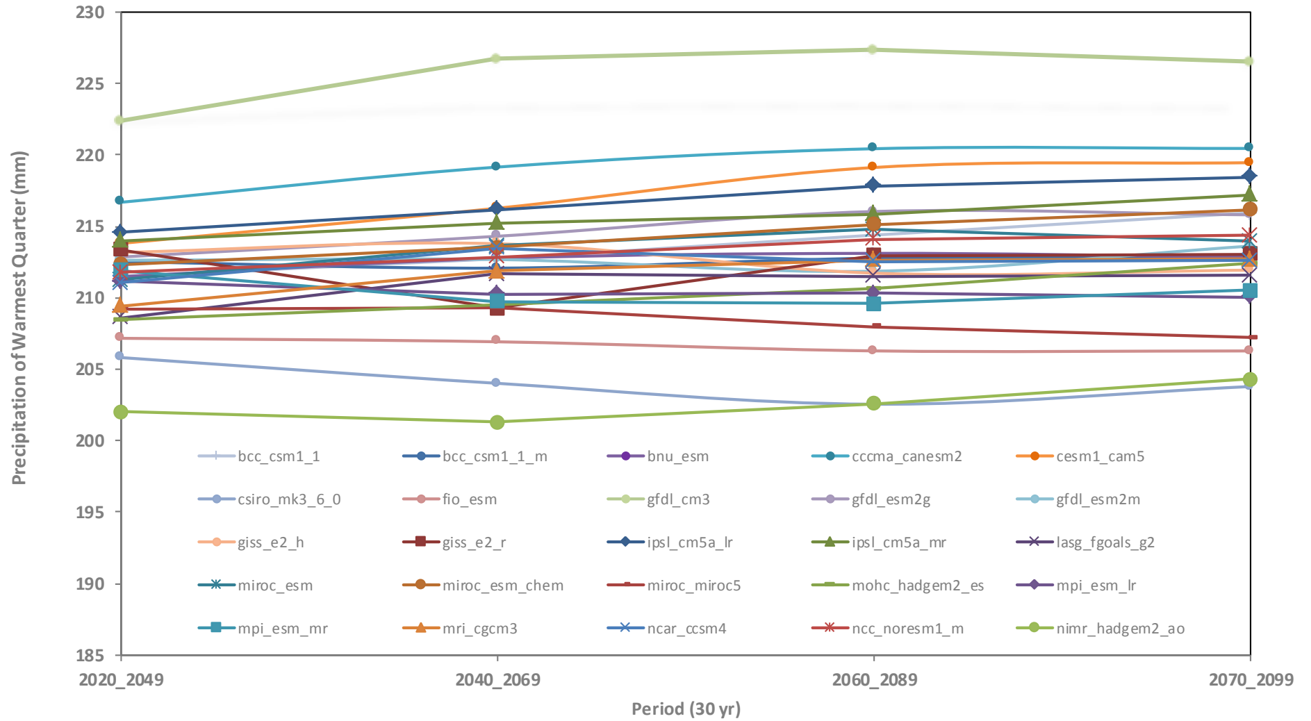
Precipitation of Warmest Quarter
