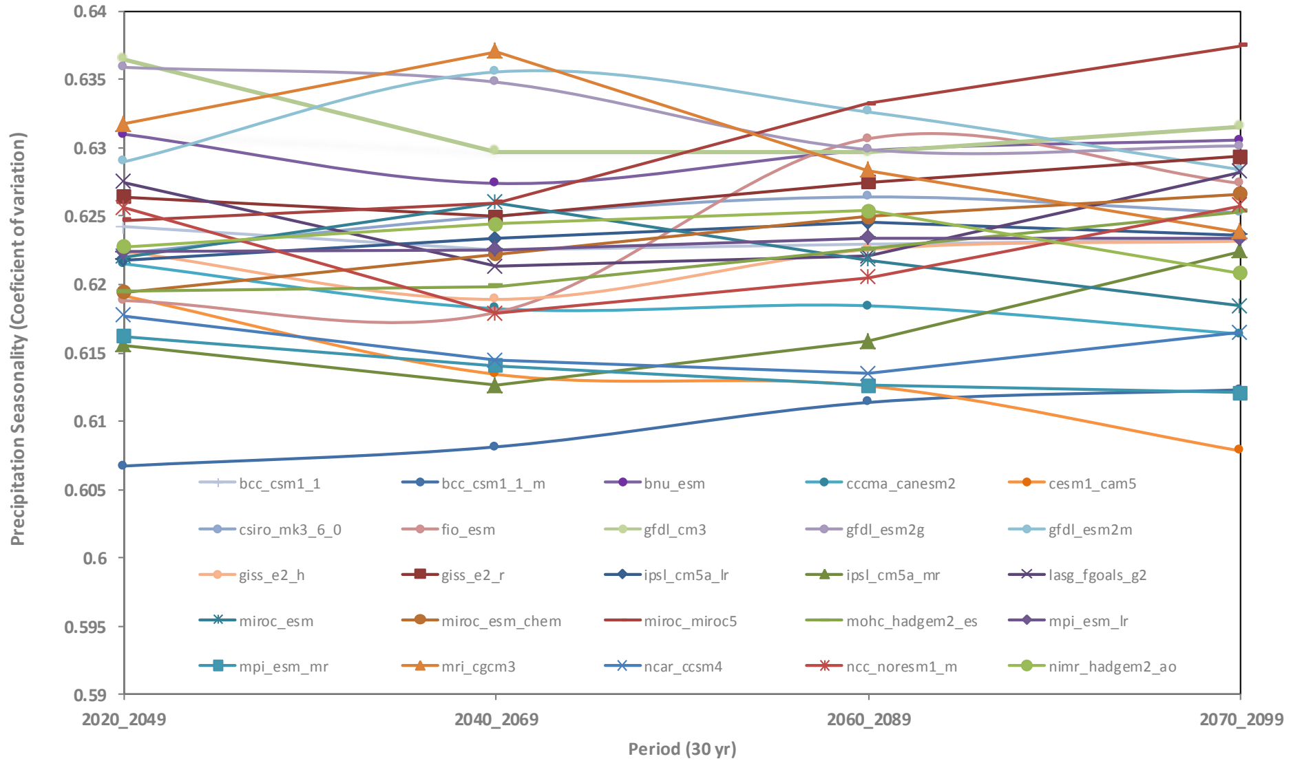
Precipitation Seasonality (Coefficient of variation)
